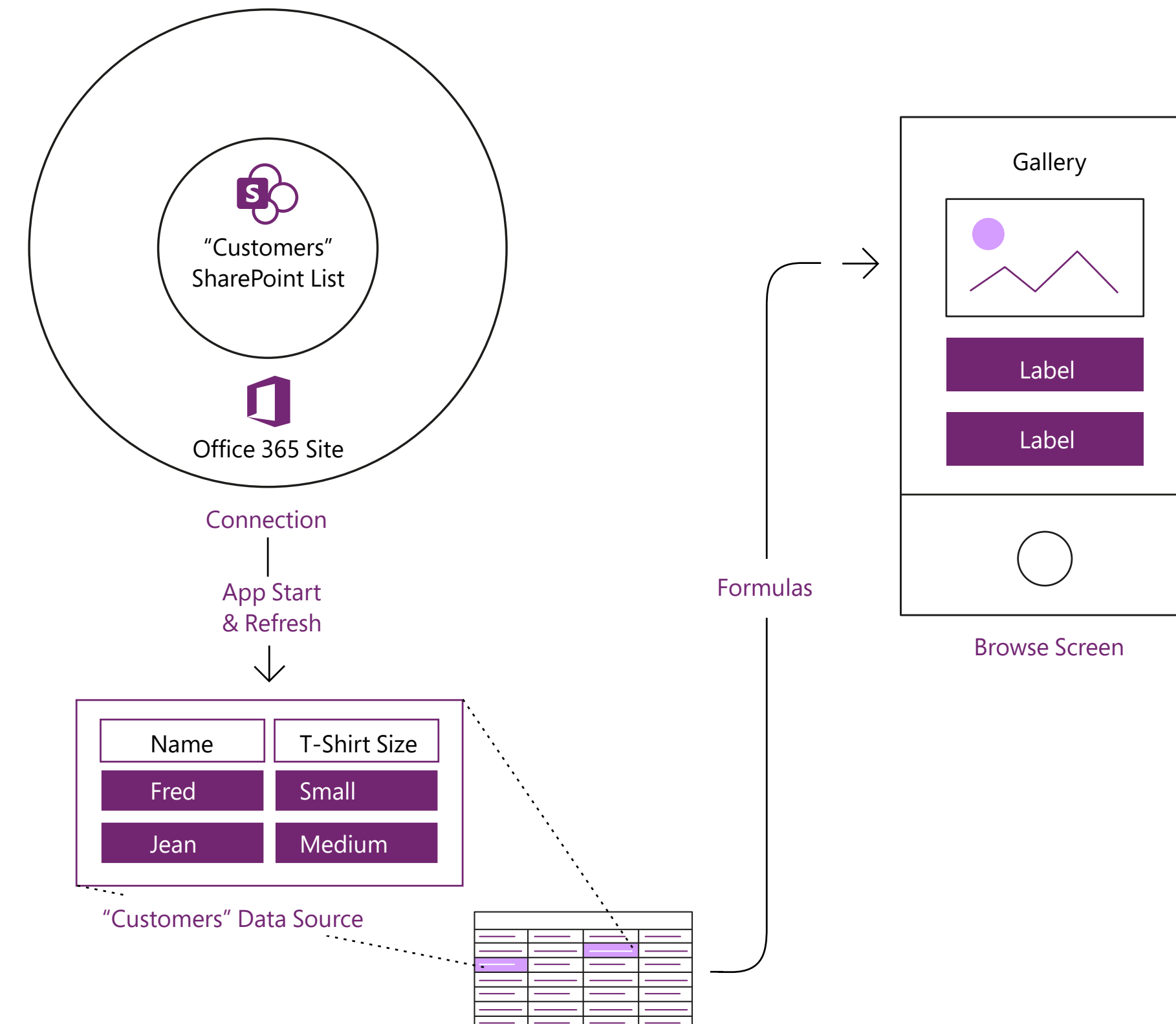
How a Canvas App pulls data from a source, in this case, a SharePoint list.
