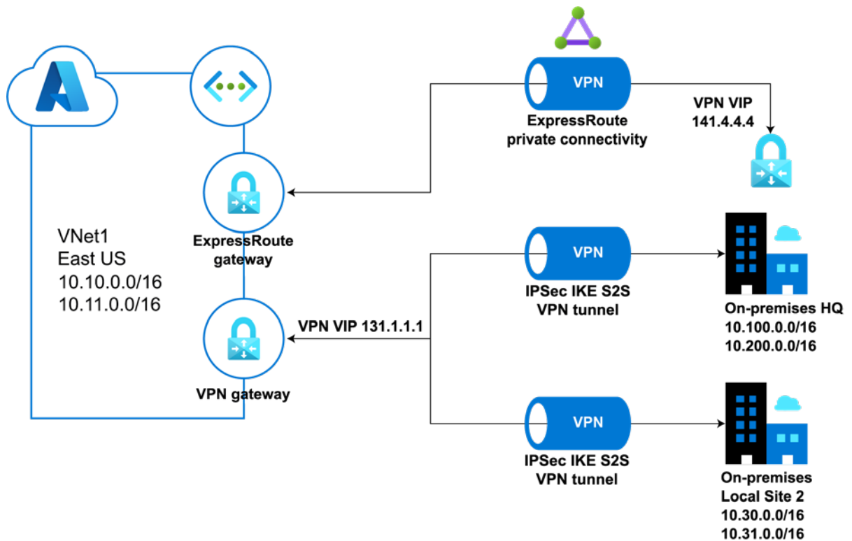
Figure 5.38: ExpressRoute
