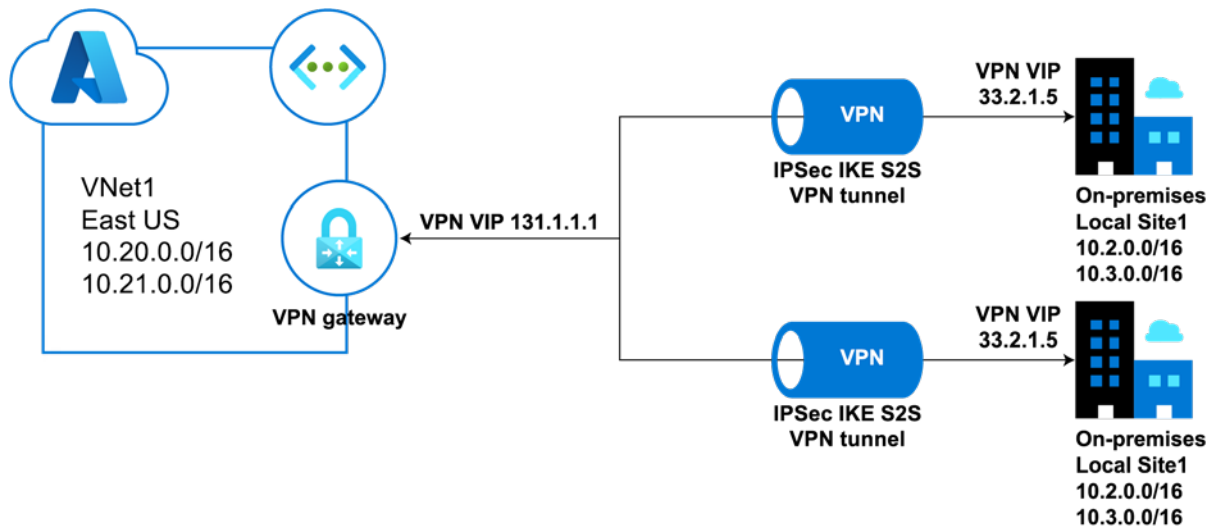
Figure 5.36: Multi-site VPN
