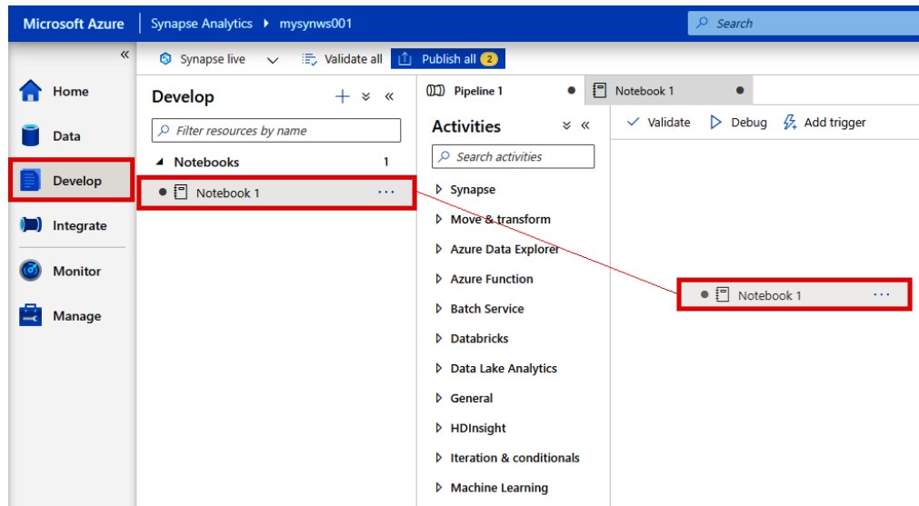
Figure 2.42: Drag an existing notebook into the pipeline
