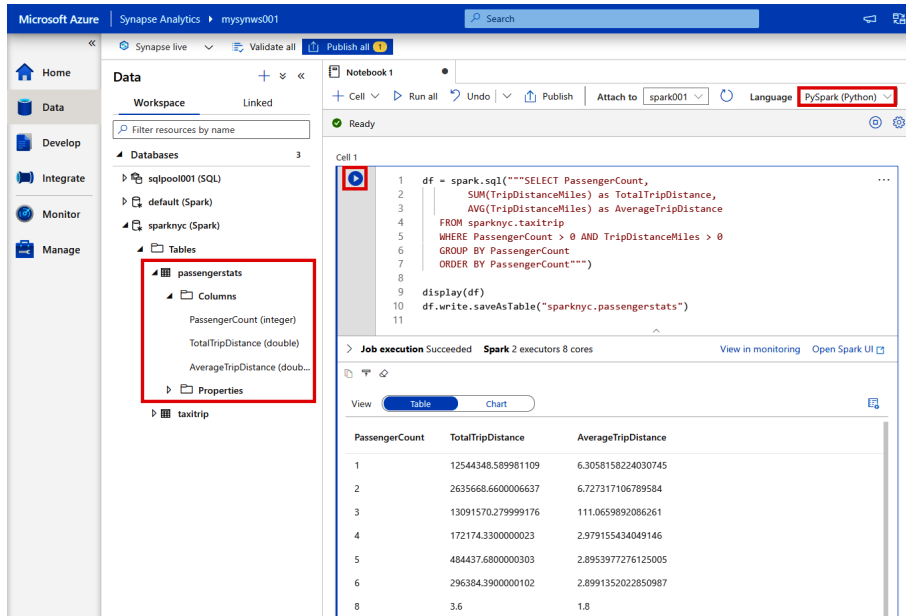
Figure 2.36: Code results
