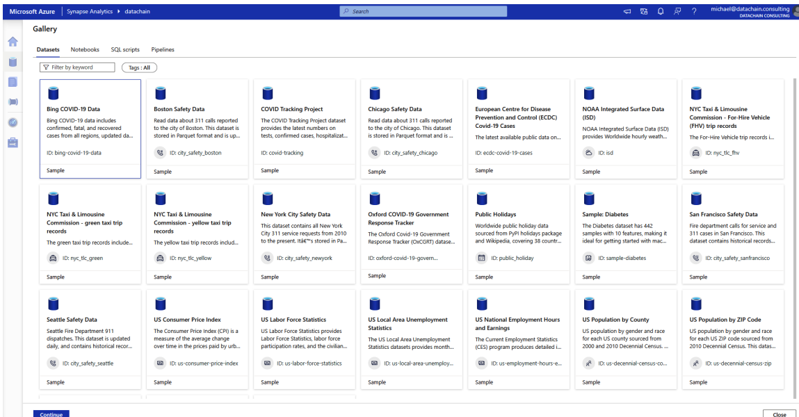
Figure 3.7: Datasets gallery
