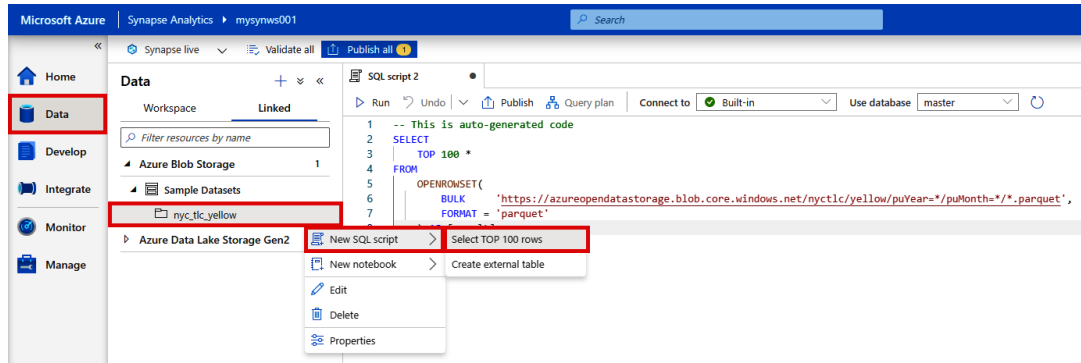
Figure 2.40: Using serverless SQL to analyze data in Azure Blob Storage
