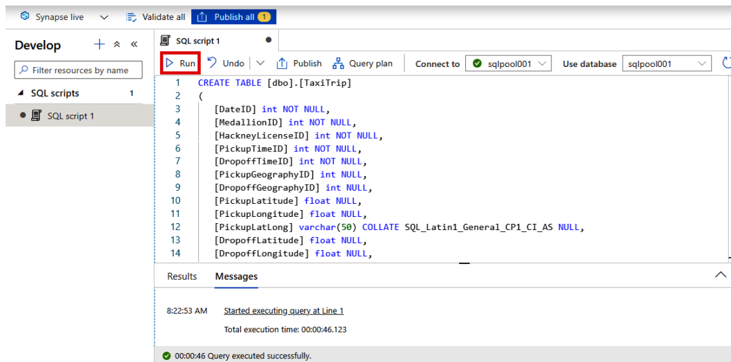
Figure 2.20: Executing the SQL script
