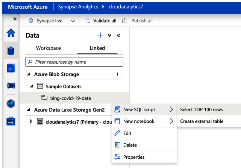
Figure 3.9: Creating a new query for selecting top100 rows
