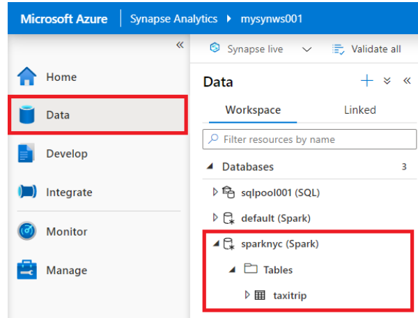
Figure 2.35: The newly created Spark database
