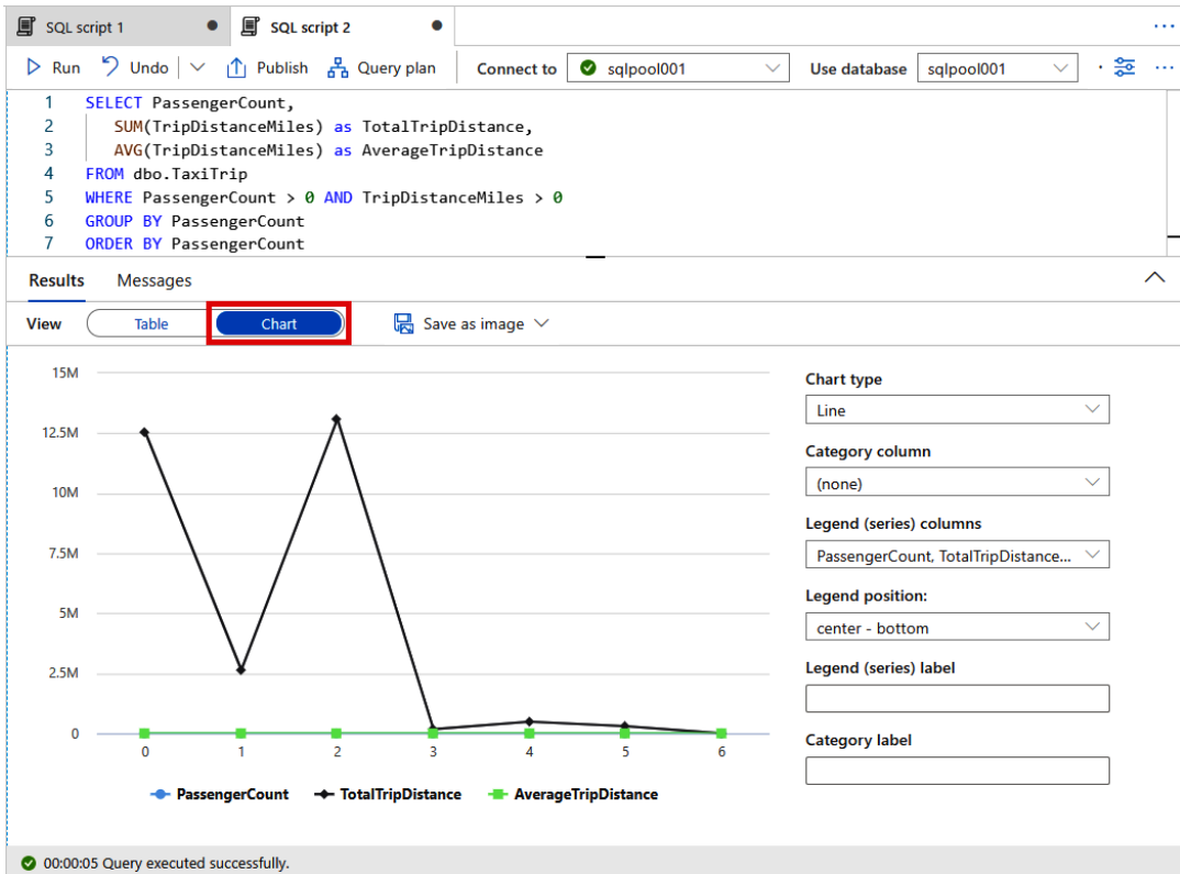
Figure 2.24: Line chart visualization
