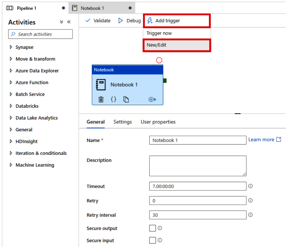
Figure 2.43: Adding a trigger
