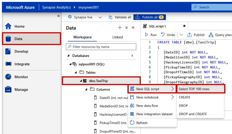
Figure 2.21: Generating a new SQL script
