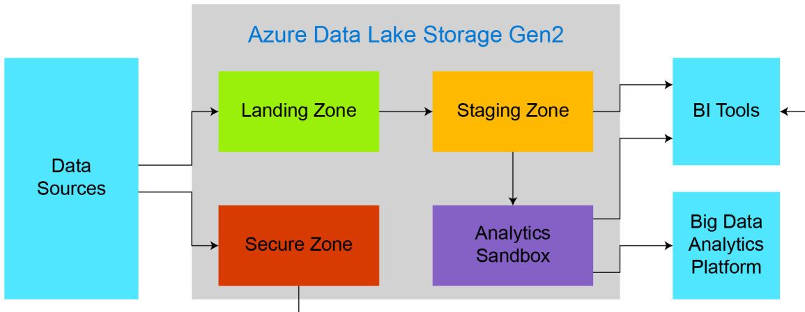
Figure 4.2: Example of data lake storage zoning
