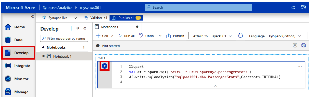
Figure 2.38: Adding a code in a notebook code cell
