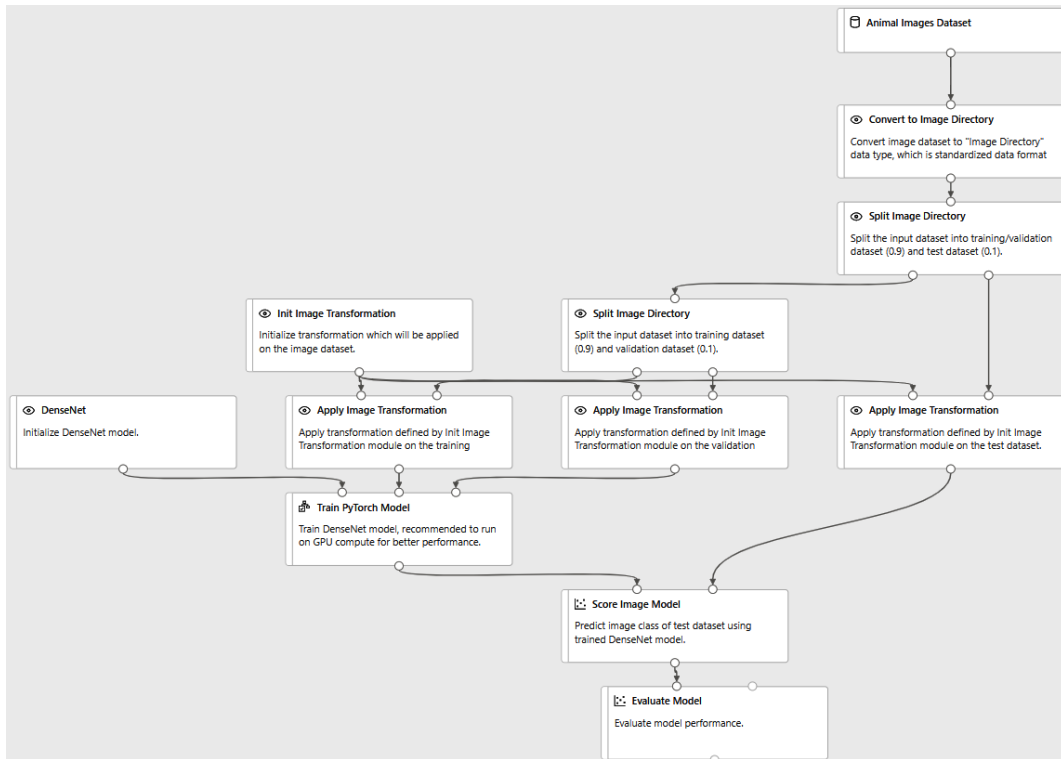
Figure 3.35: Image classification pipeline
