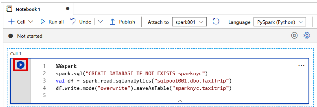
Figure 2.34: Running Spark (Scala) code to ingest SQL pool data into a Spark database
