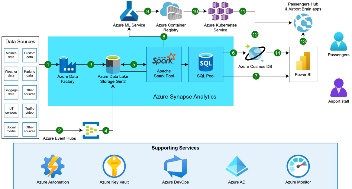
Figure 4.6: Solution architecture for NIA
