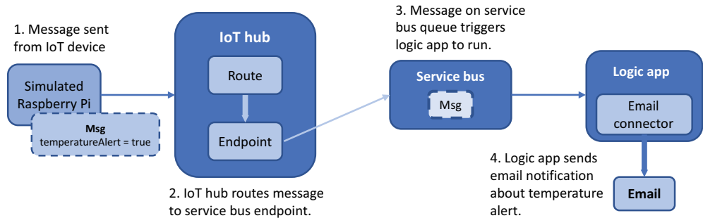
Figure 21.11 The simulated Raspberry Pi device sends a message to the IoT hub every two seconds that contains temperature sensor readings. If the temperature is above 30° C, a temperature alert is noted. The IoT hub routes any messages that contain a temperature alert to a service bus queue. Messages on this queue trigger an Azure logic app to run. The logic app is connected to an email provider, such as Outlook or Gmail, and sends an email notification about the temperature warning from the IoT device.
