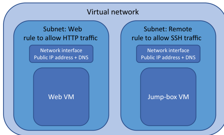
Figure 5.5 You're bringing together two subnets, NSGs, rules, network interfaces and VMs. This example is close to a production-ready deployment in which one VM runs the web server and is open to public traffic, and another VM in a separate subnet is used for remote connections to the rest of the application environment.
