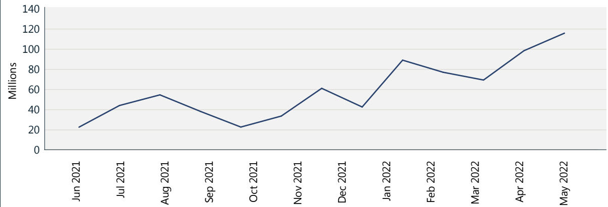
Increasing attacks on remote management ports over time, as seen through the MSTIC sensor network.
