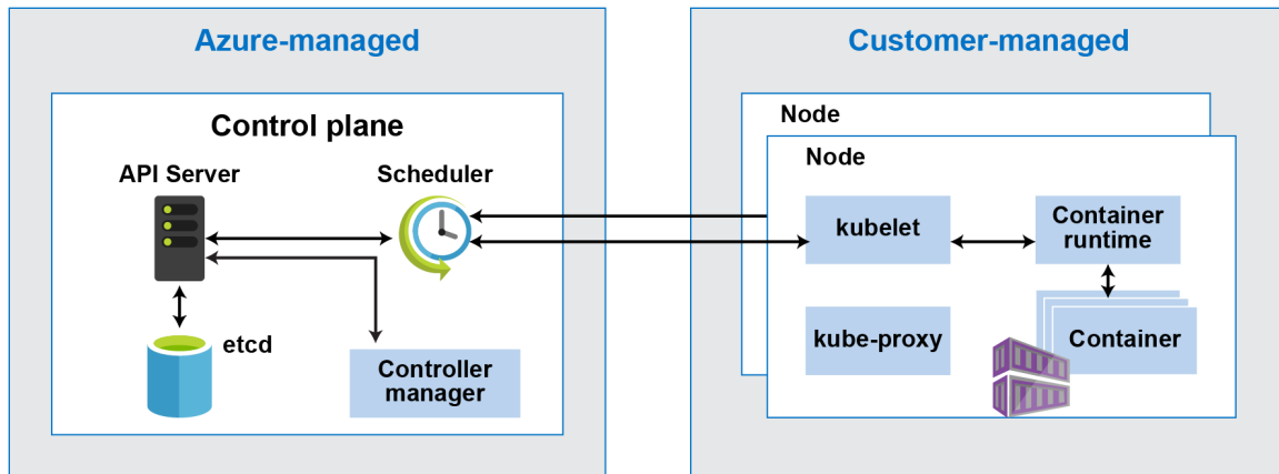
Figure 14.8: AKS architecture
