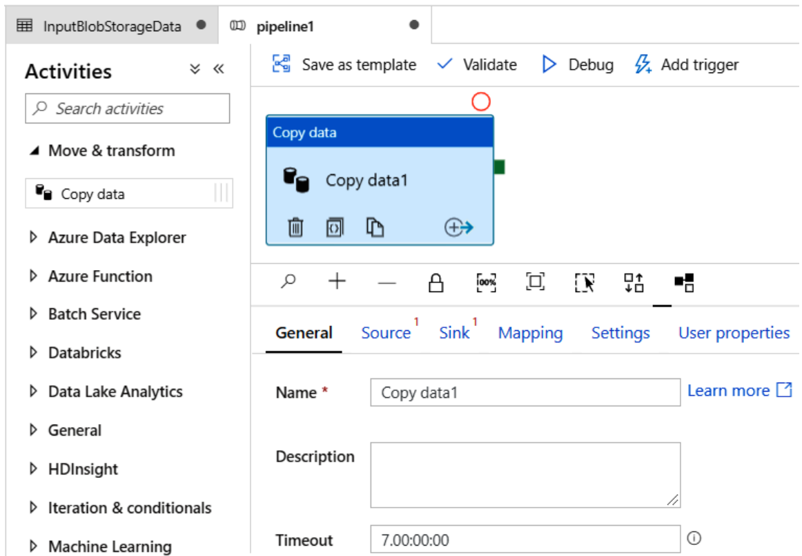
Figure 9.14: Pipeline menu
