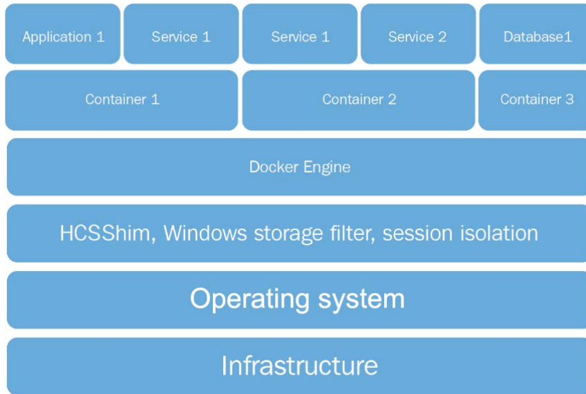
Figure 1.3: Container architecture
