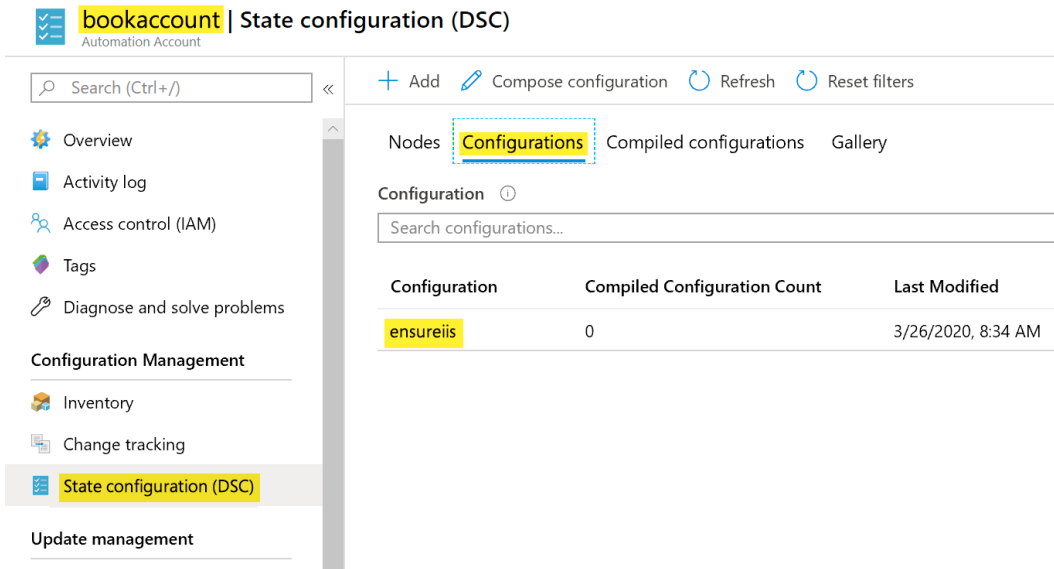
Figure 4.30: Adding configuration
