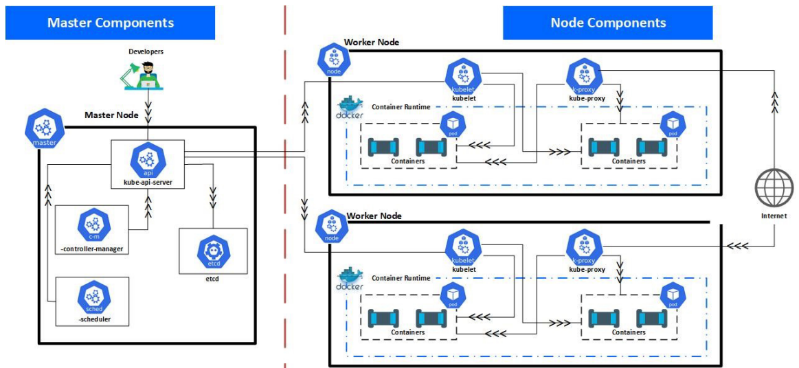
Figure 14.2: Kubernetes architecture
