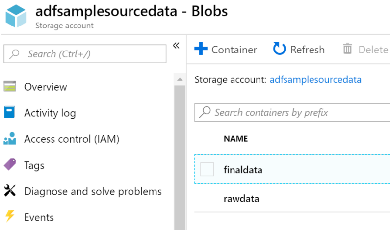
Figure 9.3: Creating containers
