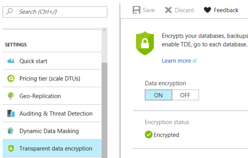
Figure 8.16: Enabling TDE
