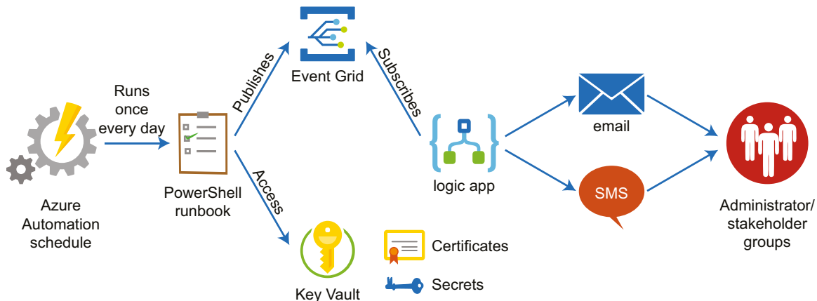
Figure 11.14: Solution architecture
