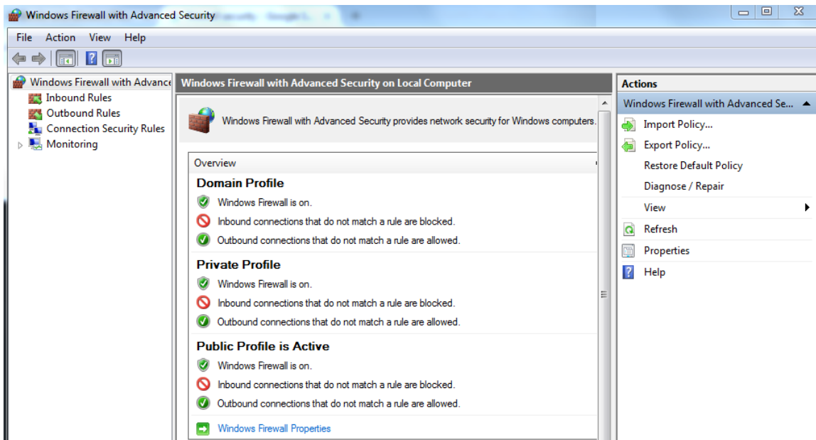
Figure 8.4: Firewall configuration
